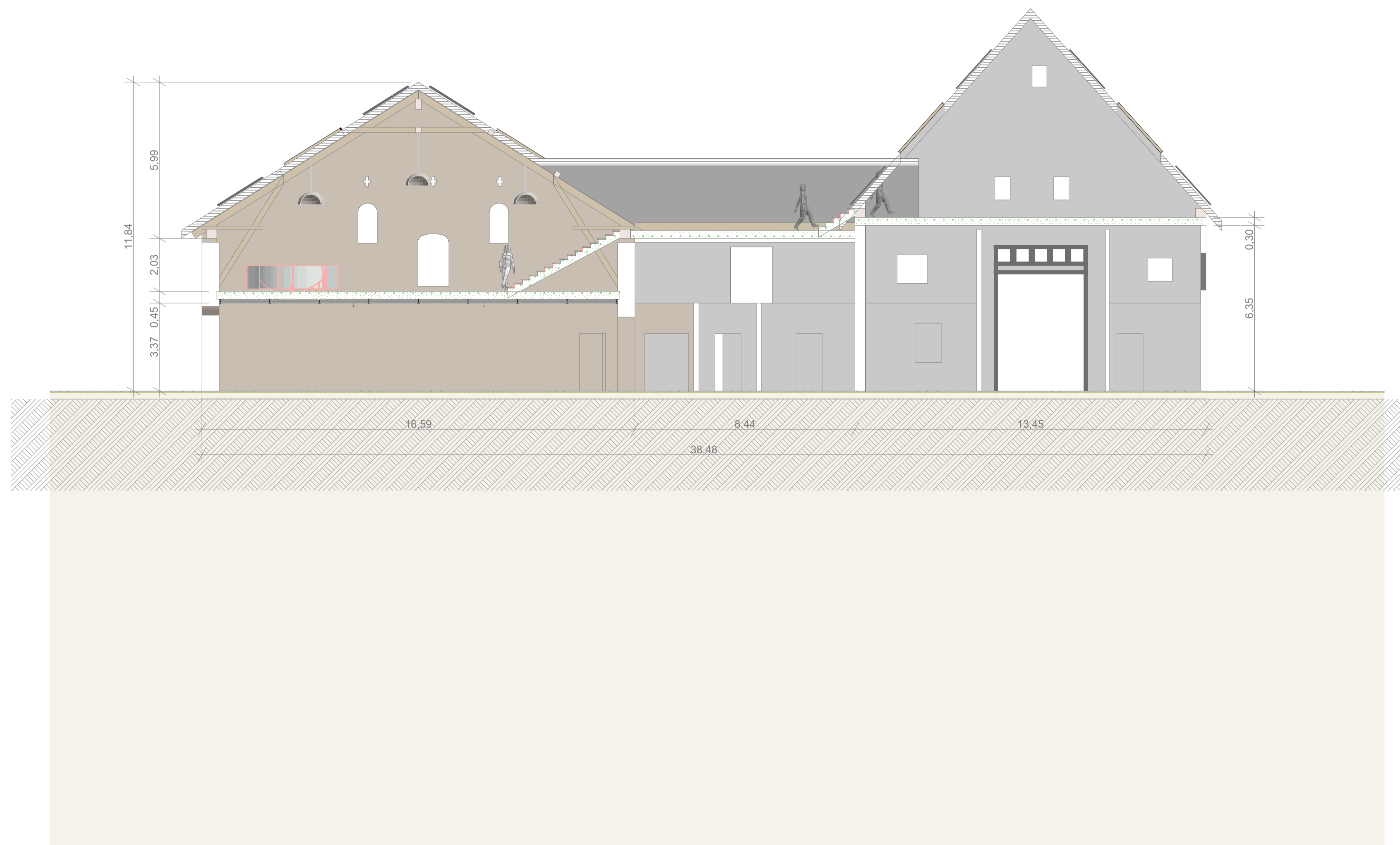
Building Section
